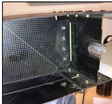
Blackhawk Stabilator
